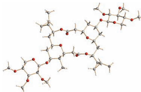
Figure 2. Molecular structure determined by X-ray diffraction. Water molecules and the secondary components of disordered atoms have been omitted for clarity.
