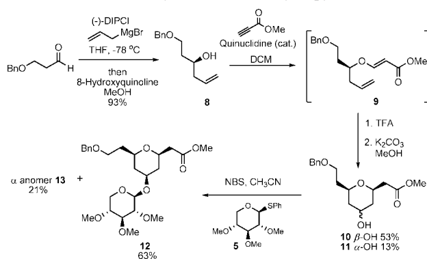
Scheme 3. Synthesis of Tetrahydropyran 12
