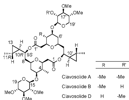
Figure 1. Clavosolides A, B, and D.
