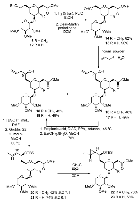
Scheme 4. Elaboration of the Side Chains
